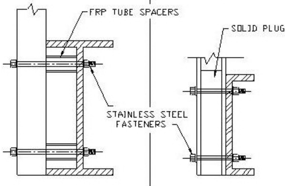
BASE MOUNT BRACKET AVAILABLE FOR STANDARD & HEAVY DUTY
