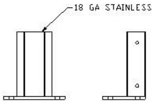
BASE MOUNT BRACKET AVAILABLE FOR STANDARD & HEAVY DUTY
